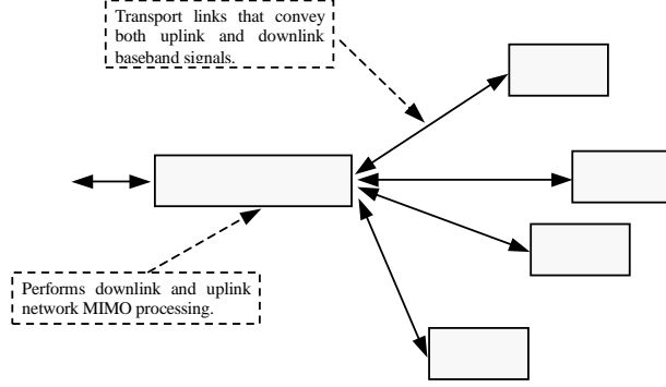
Figure 2: Transport network architecture.
