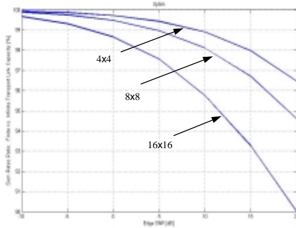
Figure 4: Uplink zero-forcing, 4x4, 8x8, and 16x16, and C_T = 16 bits/sym.
