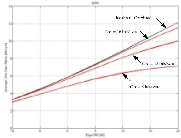
Figure 3: Uplink zero-forcing 8x8, optimal quantizer.
