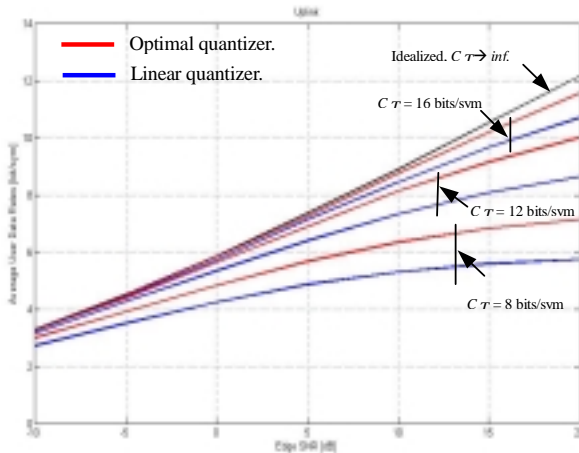
Figure 5: Uplink zero-forcing 8x8, optimal and linear quantizer.
