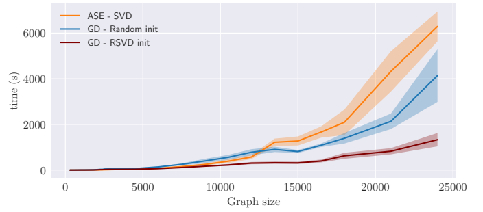
Fig. 1. Execution time for SBM graphs up to N = 24000 nodes. As N grows, GD exhibits markedly better scaling than the state-of-the-art ASE algorithm.
