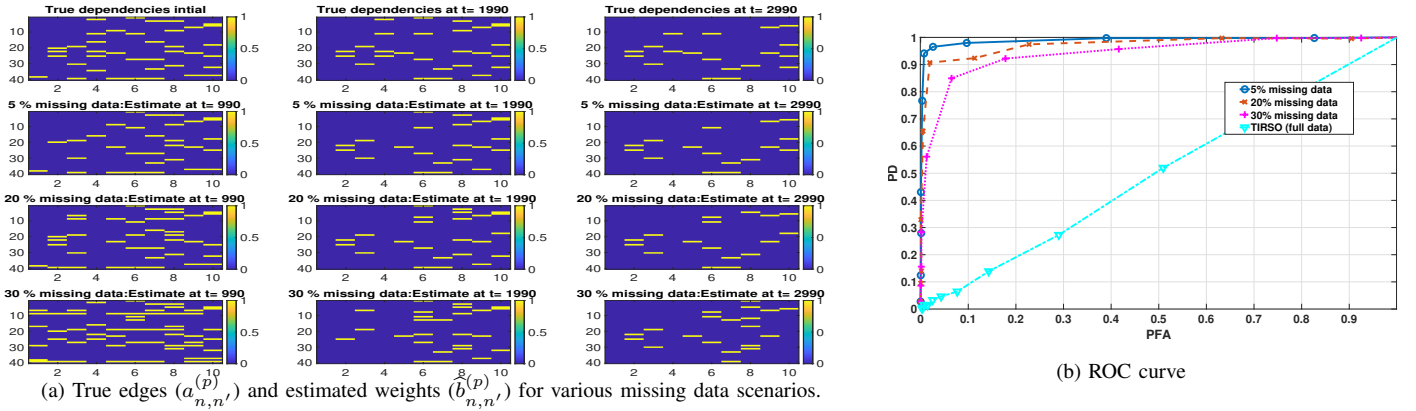
Fig. 1: Results: Experiment using synthetic data
