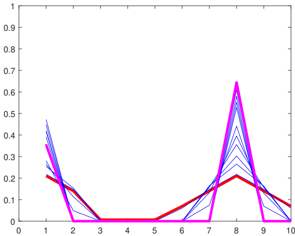
Fig. 1. Plot of super resolution O.T. method Algorithm 2. Red line is initial distribution. Blue lines are steps along gradient of Equation (7). Pink line is final, converged distribution. \lambda = 10 . epsilon = 0.1. Max Sinkhorn iterations = 5000. Gradient step size = 0.01. Gradient steps=50.
