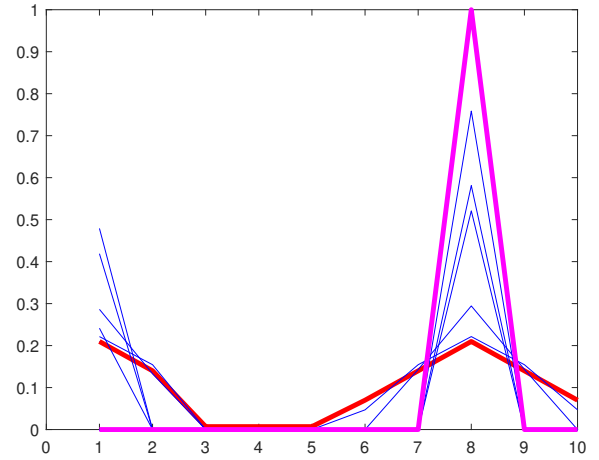
Fig. 2. Plot of super resolution O.T. method Algorithm 2. Red line is initial distribution. Blue lines are steps along gradient of Equation (7). Pink line is final, converged distribution. \lambda = 100 . epsilon = 0.1. Max Sinkhorn iterations = 5000. Gradient step size = 0.01. Gradient steps=50.
