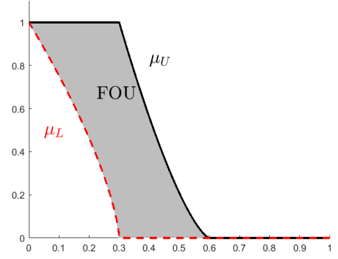
(b) Piecewise nonlinear membership function ( 0 < \alpha_{j,L}, \alpha_{j,U} < 1 in (3-4))
