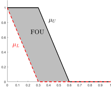
(a) Piecewise linear membership function ( \alpha_{j,L} = \alpha_{j,U} = 1 in (3-4))
