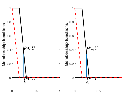
(a) Evaluating uncertainty based on VAE's error using the piecewise linear membership
