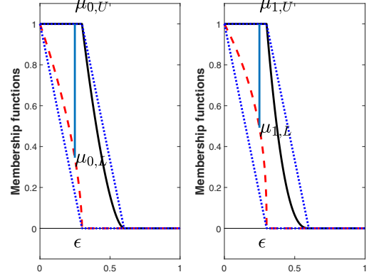
(b) Evaluating uncertainty based on primary membership using the piecewise nonlinear membership function
